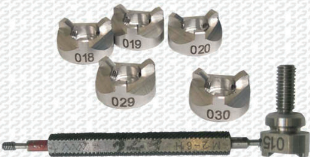
Measuring adapters
